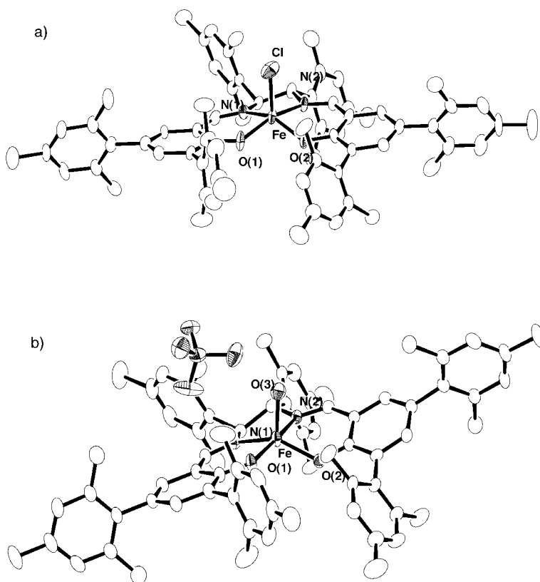
Figure 1. Thermal-ellipsoid plots (50 % probability) of a) 2 and b) 3 . Hydrogen atoms and solvents of crystallization have been omitted for clarity. Selected bond distances [Å] and angles [°]: 2 : Fe–Cl 2.234(3), Fe–O(1) 1.881(6), Fe–O(2) 1.878(5), Fe–N(1) 2.102(6), Fe–N(2) 2.087(6); O(1)–Fe–N(2) 154.1(3), O(2)–Fe–N(1) 143.3(3). 3 : Fe–O(1) 1.863(3), Fe–O(2) 1.876(3), Fe–O(3) 2.009(3), Fe–N(1) 2.084(3), Fe–N(2) 2.060(3); O(1)–Fe–N(2) 166.6(1), O(2)–Fe–N(1) 137.7(1).
